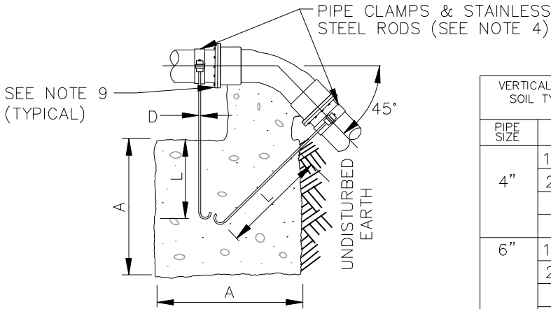
VERTICAL BLOCKING FOR 45° BENDS
