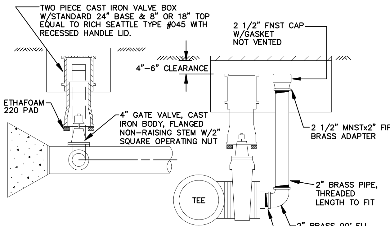
SIDE VIEW (PROFILE)
