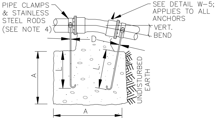
VERTICAL BLOCKING 11 1/4° & 22 1/2° BENDS
