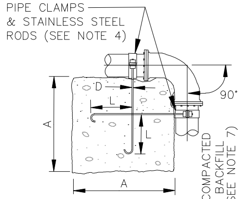
VERTICAL BLOCKING FOR 90° BENDS (SEE NOTE 6)
