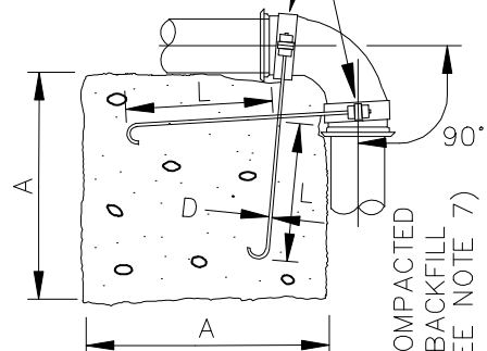
VERTICAL BLOCKING FOR 90° BENDS (SEE NOTE 6)
