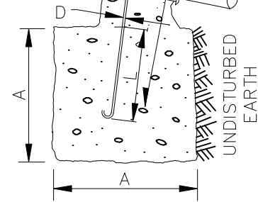
VERTICAL BLOCKING 11 1/4° & 22 1/2° BENDS
