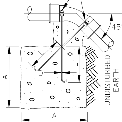
VERTICAL BLOCKING FOR 45° BENDS
