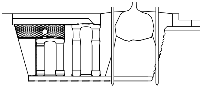
A. UTILITY ON TOP SOIL CELL DECK
