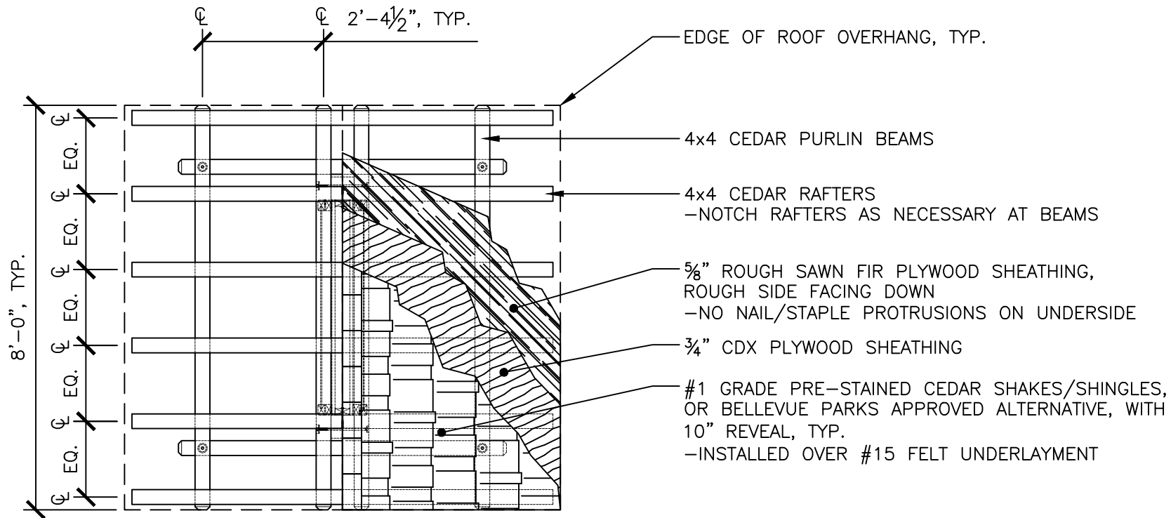
ROOF LAYOUT
