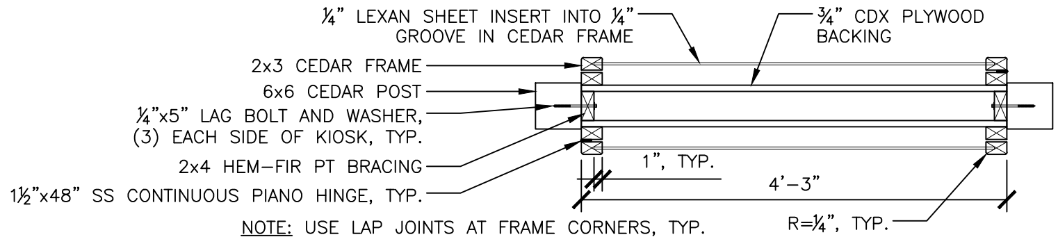
DISPLAY CASE SECTION
