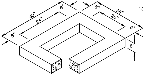
6" REDUCING SECTION
