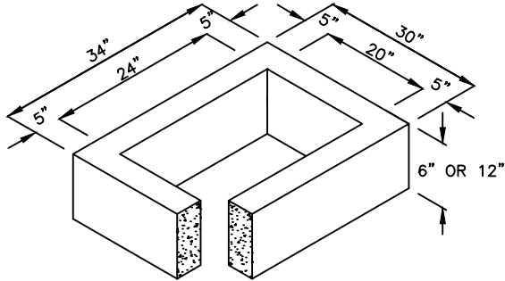
RISER SECTION
