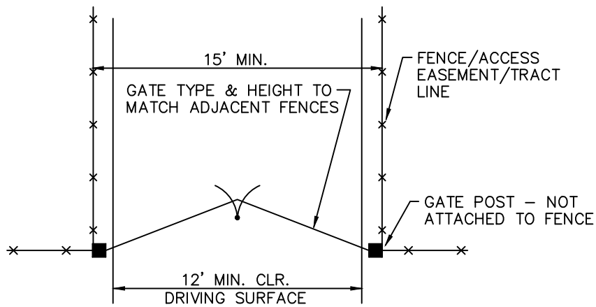
GATE PLACEMENT
