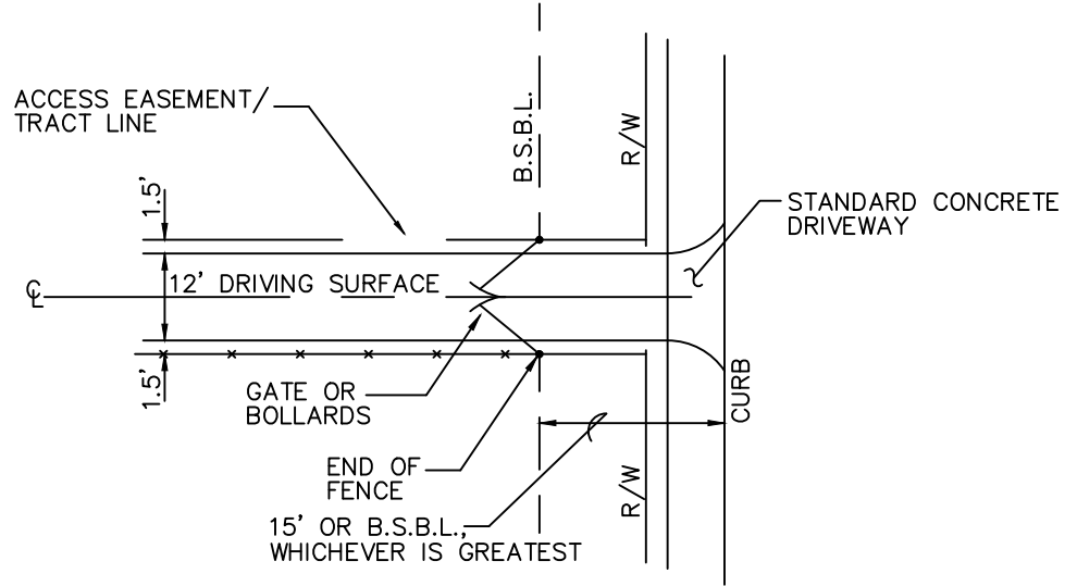
DRIVEWAY ENTRANCE
