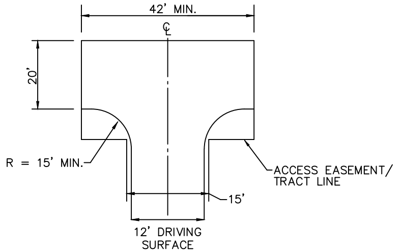
HAMMERHEAD
