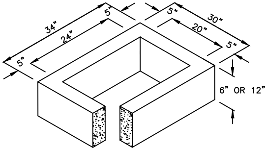
RISER SECTION
