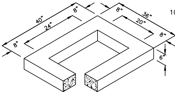
6" REDUCING SECTION
