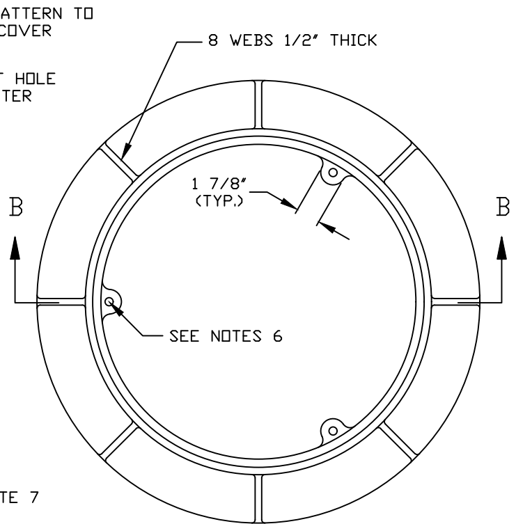
RING PLAN
