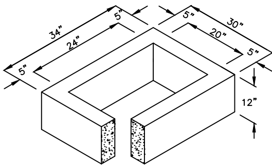
12" RISER SECTION
