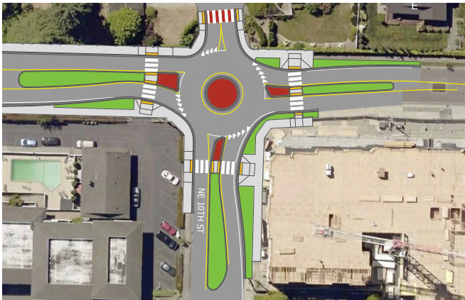
Rendering of a mini-roundabout at 100th Avenue NE and NE 10th Street | 在100th Avenue NE 和 NE 10th Street 设立迷你环形交叉路
