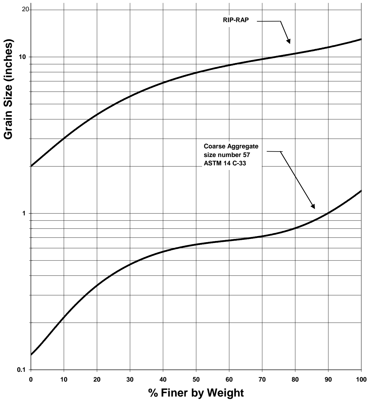
Figure 4.2 Riprap/Filter Example Gradation Curve
