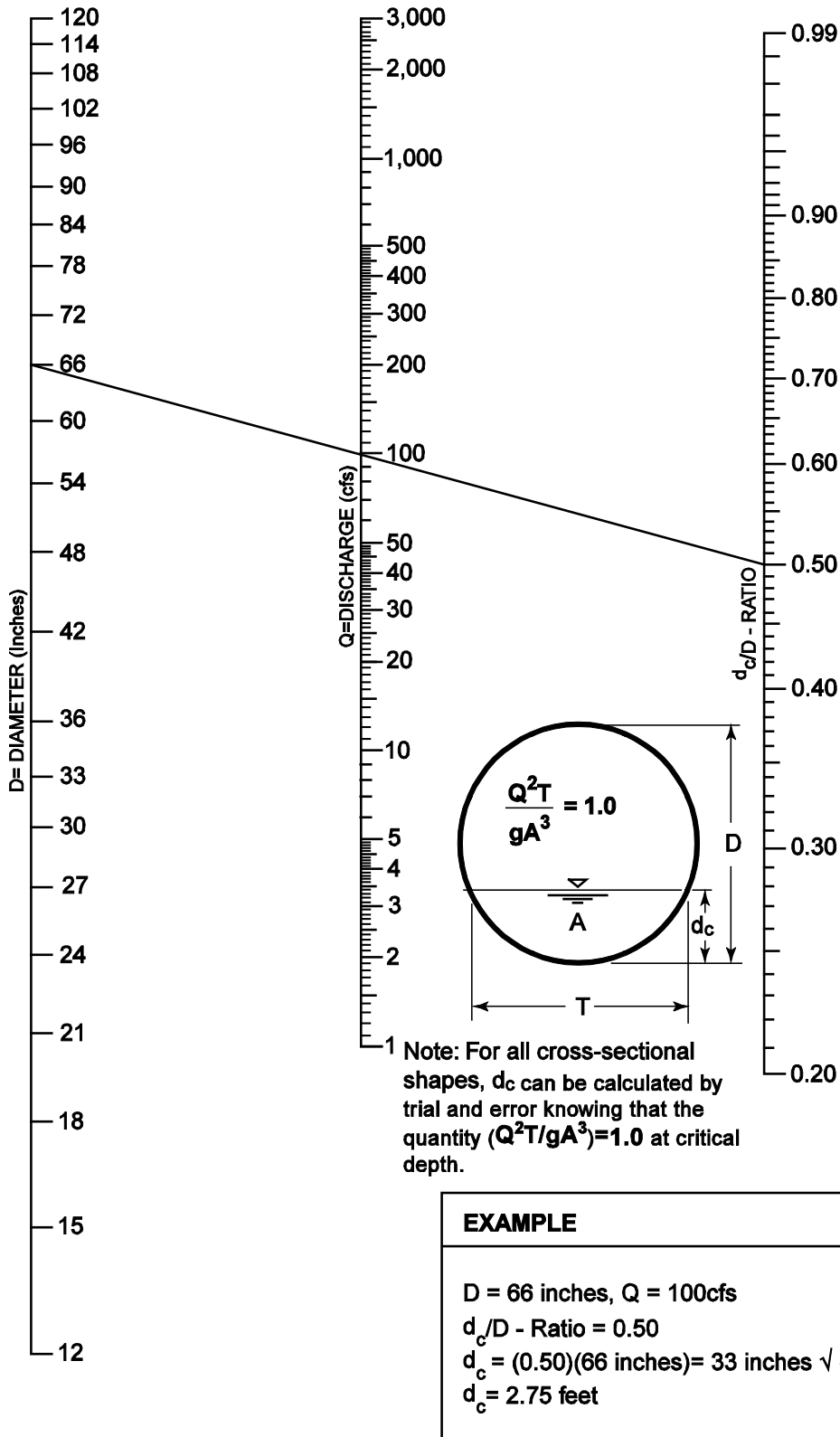
Figure 4.14 Critical Depth Of Flow For Circular Culverts
