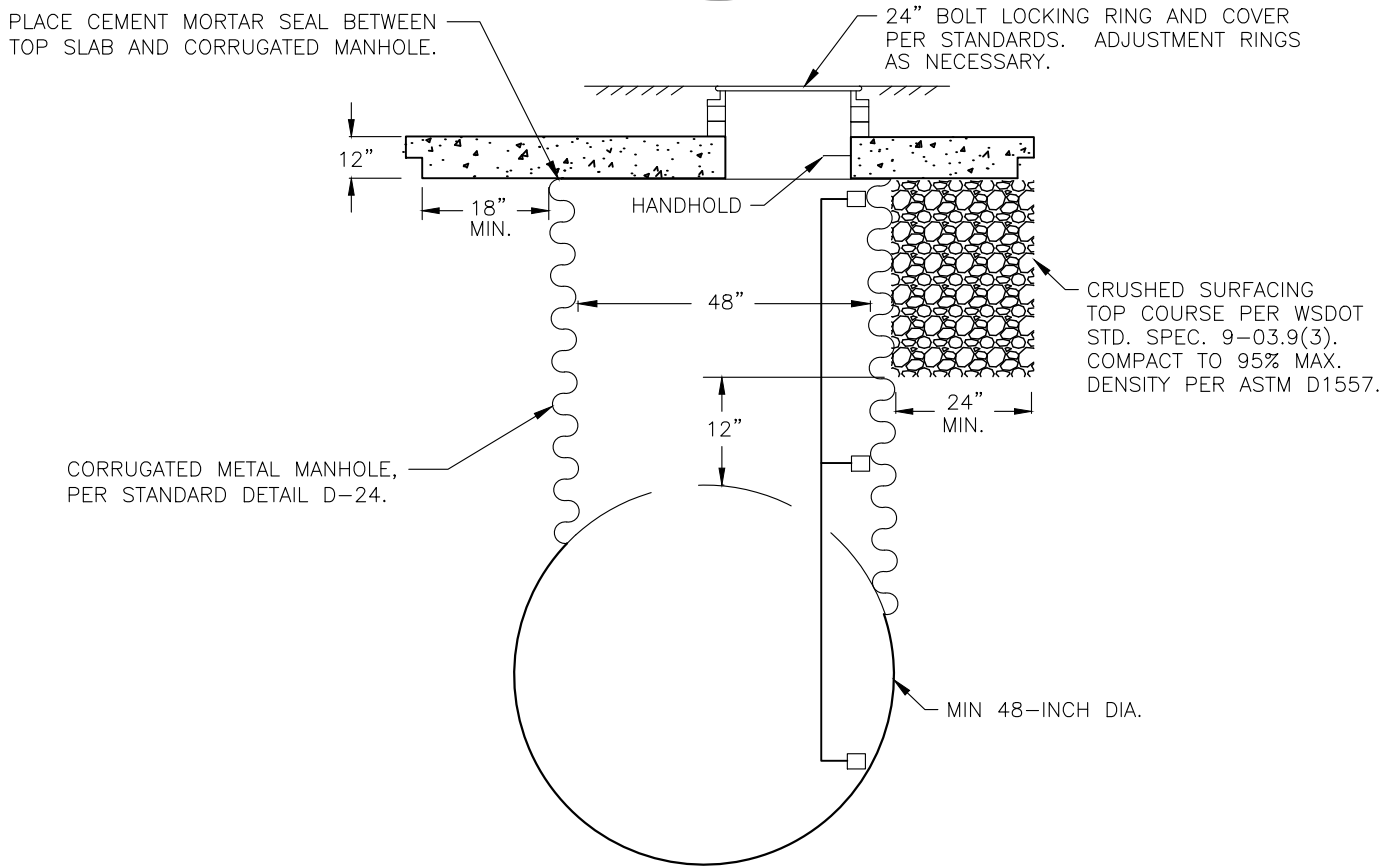
ECCENTRIC SECTION
