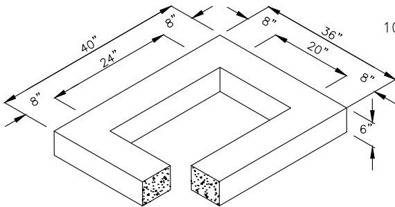
6" REDUCING SECTION
