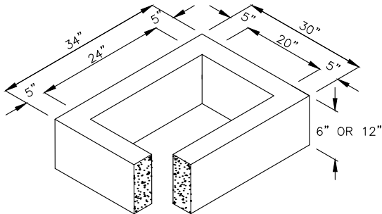
RISER SECTION
