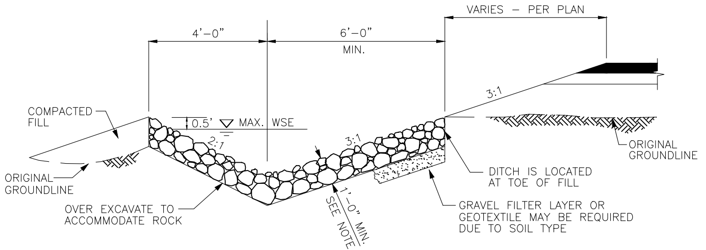
ROCK-LINED SHOULDER DITCH IN FILL SECTION
