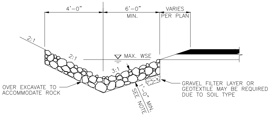
ROCK-LINED SHOULDER DITCH IN CUT SECTION
