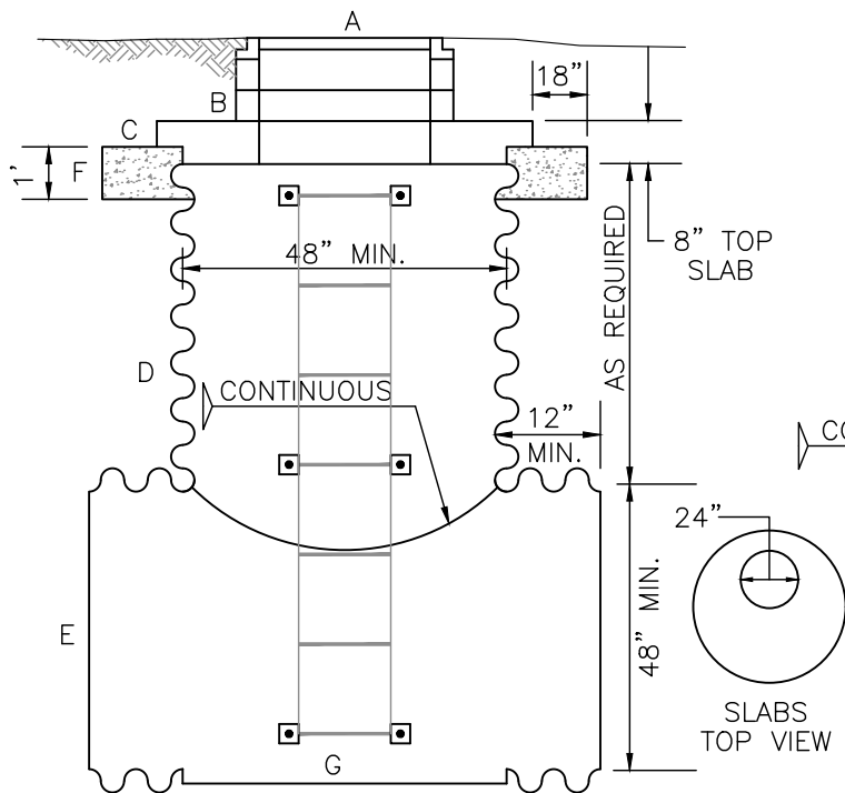
CONCENTRIC ELEVATION
