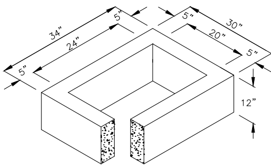
12" RISER SECTION
