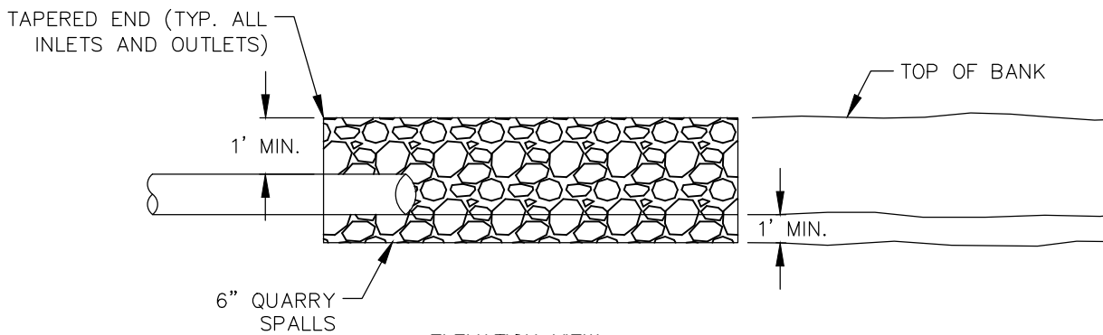
ELEVATION VIEW
