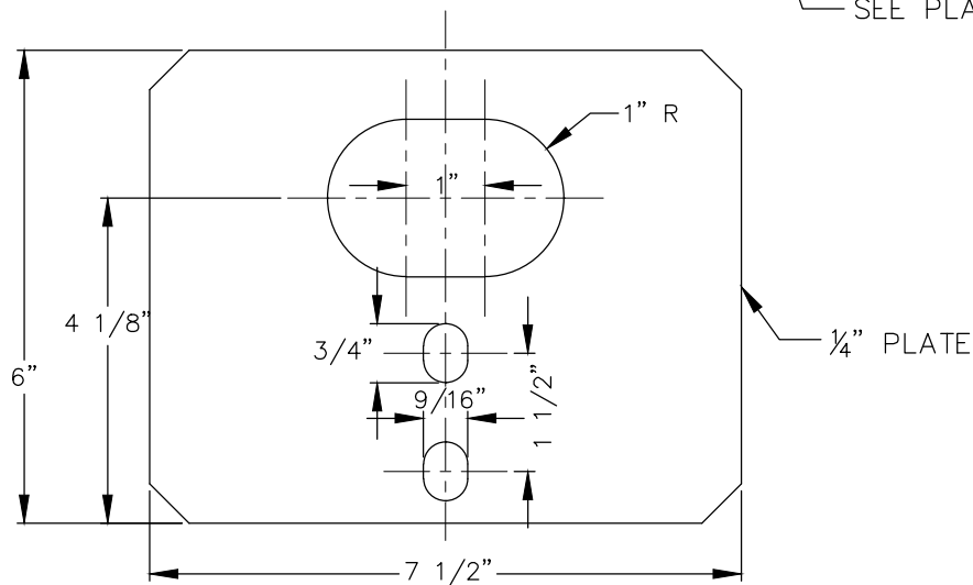
PLATE DETAIL
