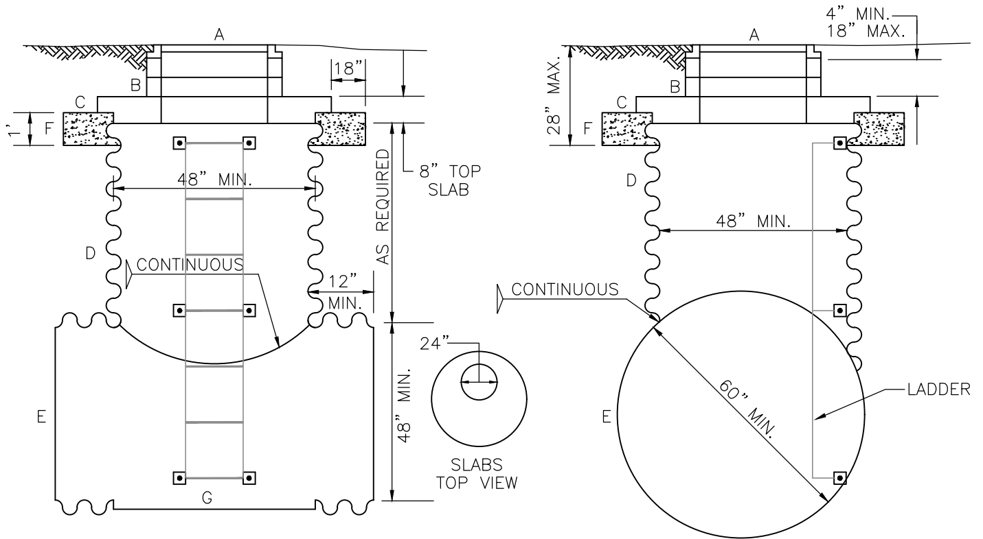
CONCENTRIC ELEVATION
