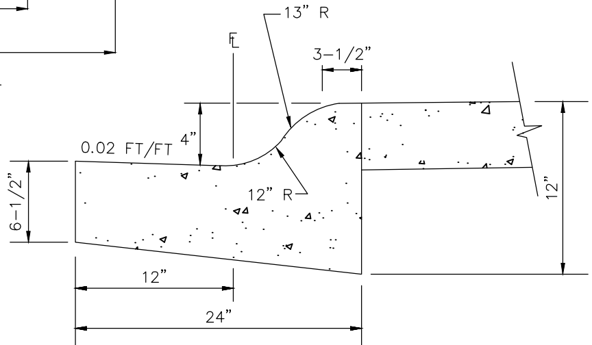
ROLLED CURB
