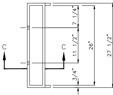
HOOD DETAIL
