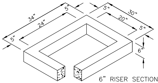
6" RISER SECTION
