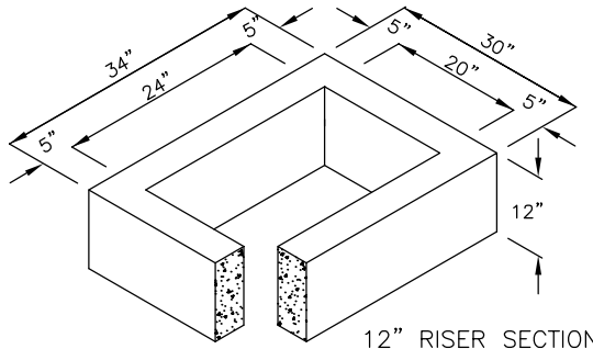
12" RISER SECTION
