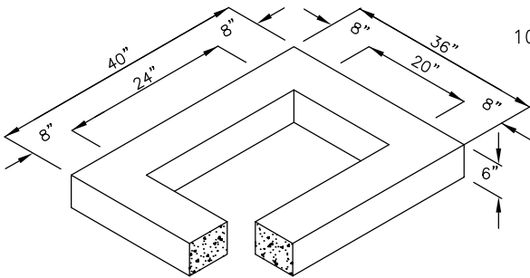
6" REDUCING SECTION
