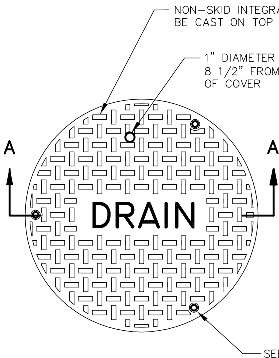
COVER PLAN
