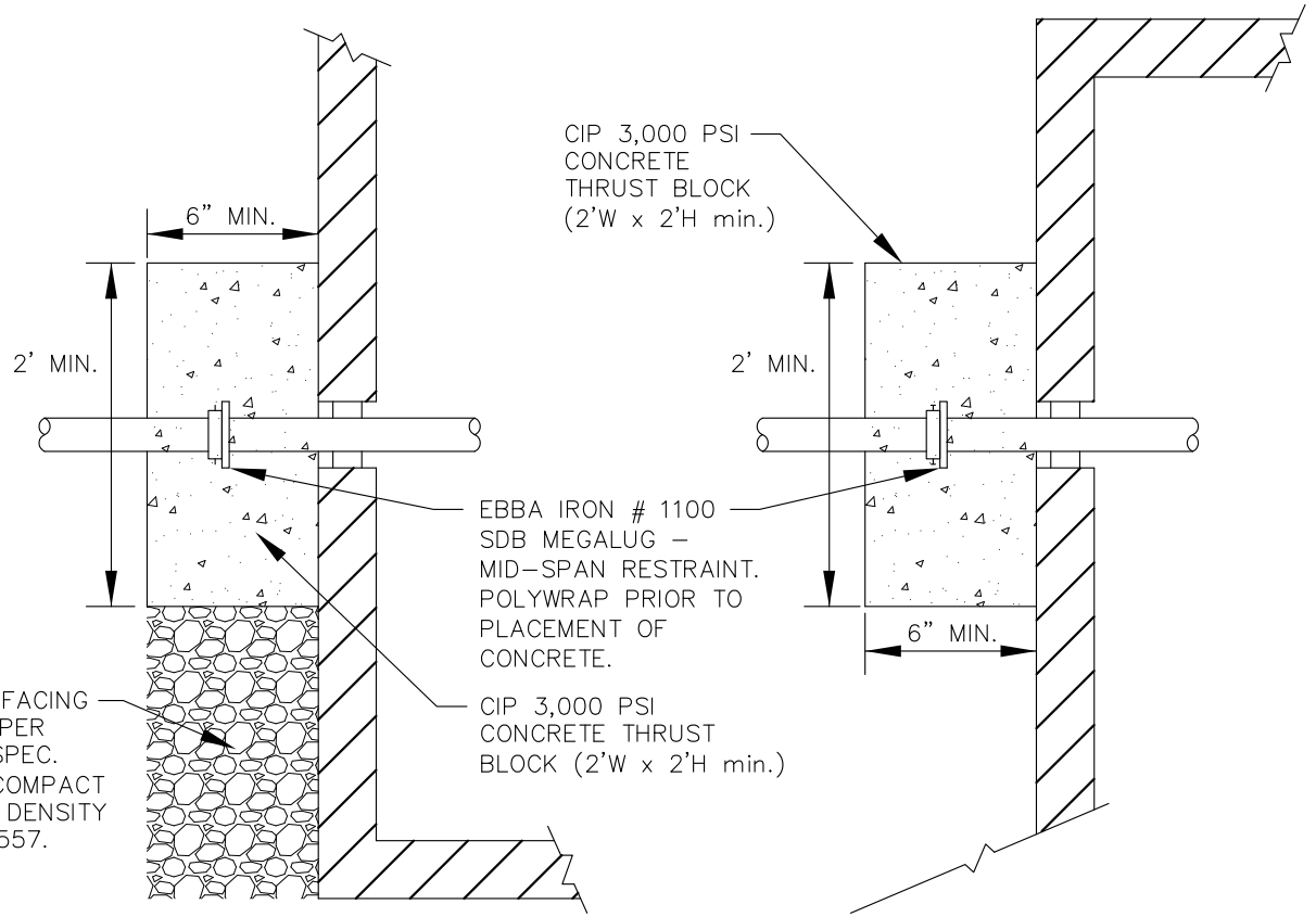
PROFILE
