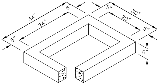
6" RISER SECTION
