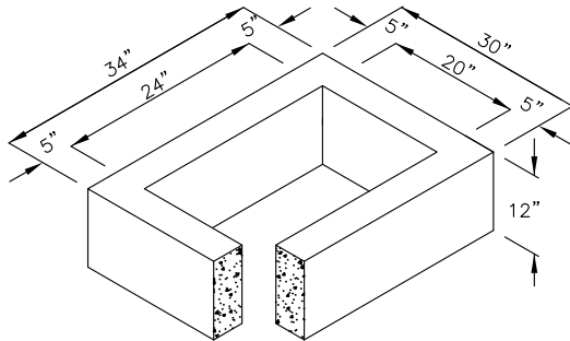
12" RISER SECTION
