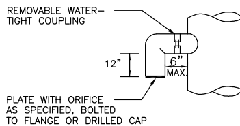
ELBOW DETAIL
