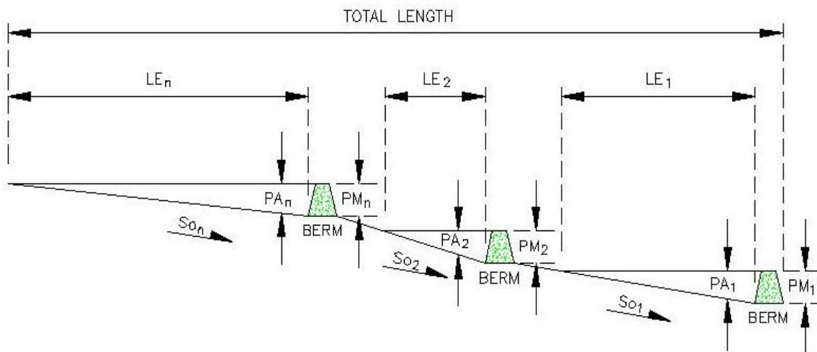
Figure 6.2. Schematic for calculating Bottom Length and Effective Total Depth for bioretention or pervious pavement on slopes where check dams (berms) are used. Refer to
