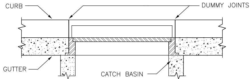
SECTION B-B
