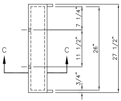
HOOD DETAIL
