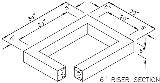
6" RISER SECTION
