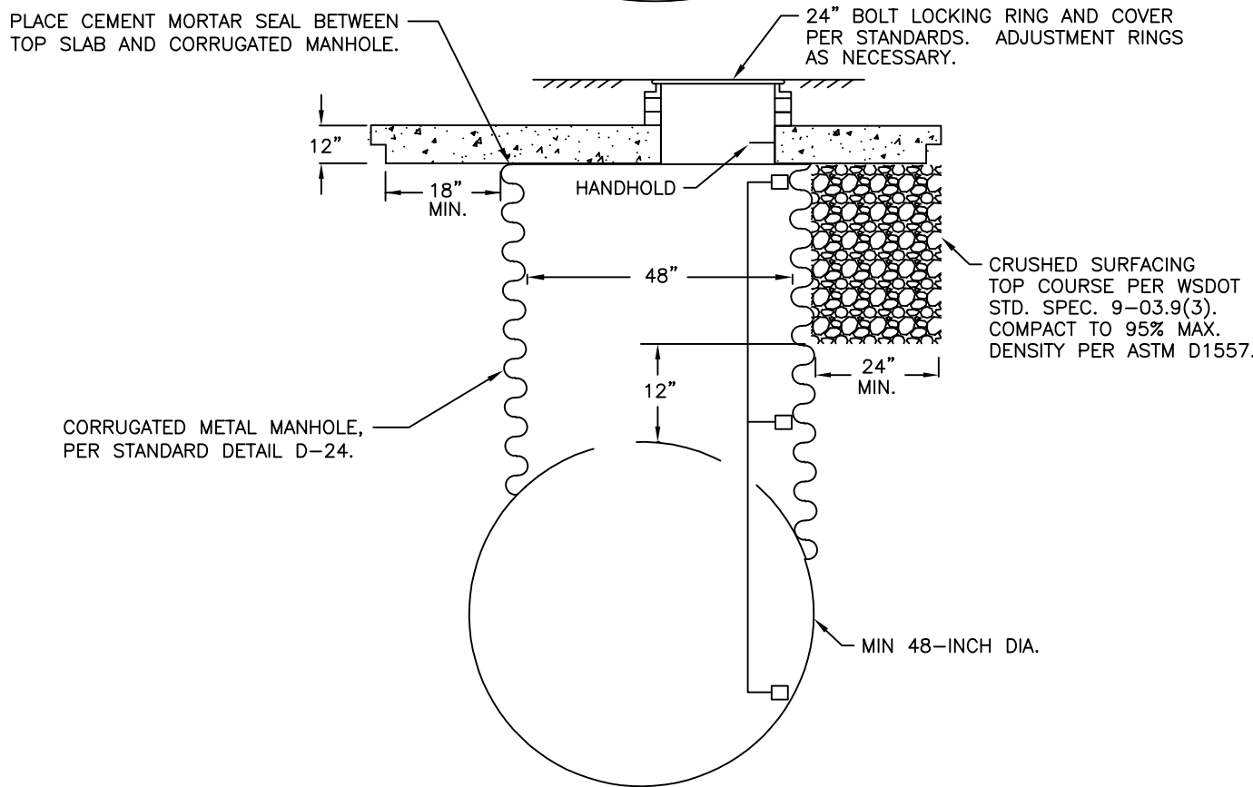
ECCENTRIC SECTION
