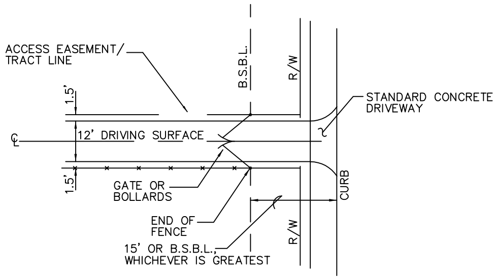
DRIVEWAY ENTRANCE
