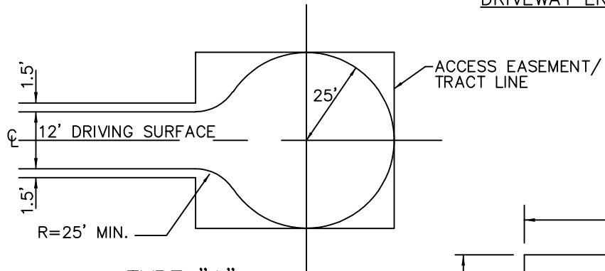
TYPE "A" TURNAROUND
